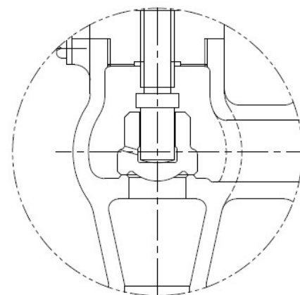
CHECK VALVE
